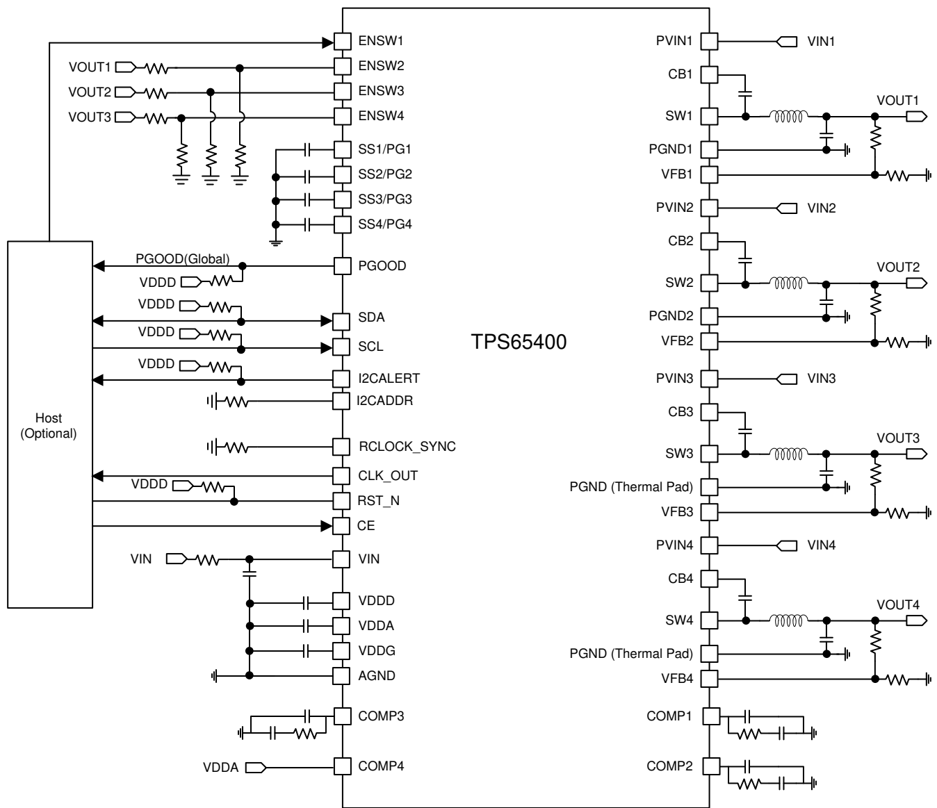
Figure 9-13. External Sequencing Schematic, \overline{\text{VOUT}} > \text{VEN}
